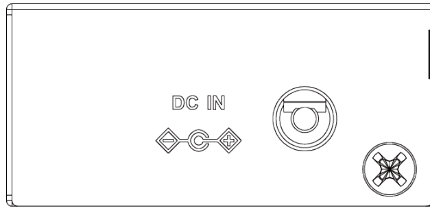
Figure 1-4 Side panel (8-port)
